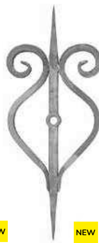
Forgiato / Forged H. 800 x L. 315 mm Art. 15.255 □ 30 mm
