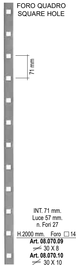
FORO QUADRO SQUARE HOLE
