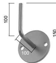
Piastra/Plate Ø 100 ≠ 8 mm. Art. 15.003.08 Ø 10 mm. forata / holed
